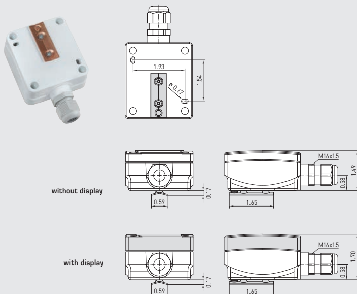
Dimensional drawing [inch]
