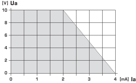
Dependency of output current on output voltage
