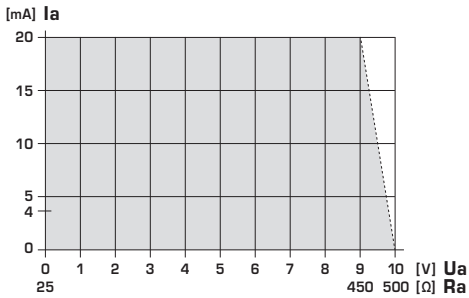
Dependency of output voltage on output current
