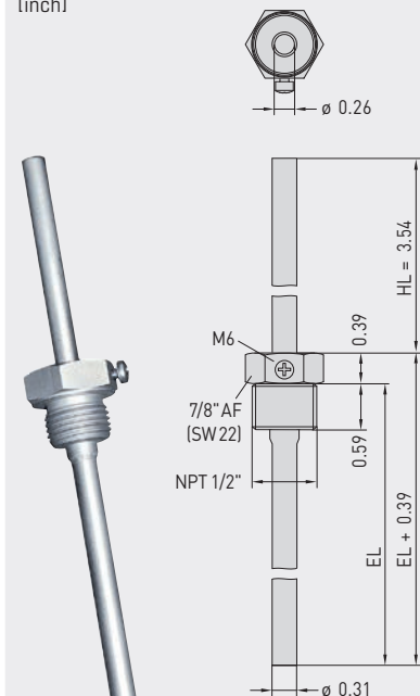
Dimensional drawing [inch]
